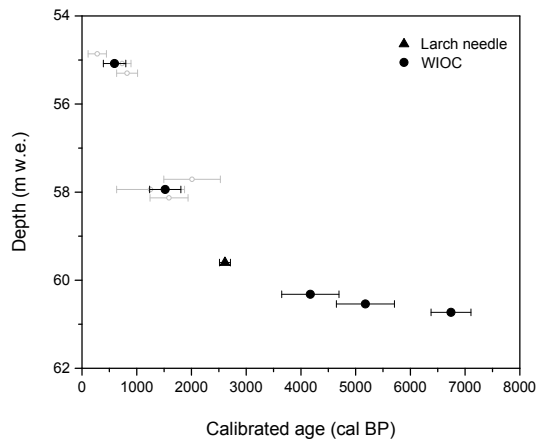
Figure 5. Dating of the bottom part of the Ortles ice core. Circles indicate the ages derived with the WIOC ^{14}\text{C} method and the triangle shows the age of the conventionally ^{14}\text{C} dated larch leaf found in the ice core (Gabrielli et al., 2016). Light grey circles show the ages obtained for the subsamples. Errors bars represent the 1\sigma uncertainty.
