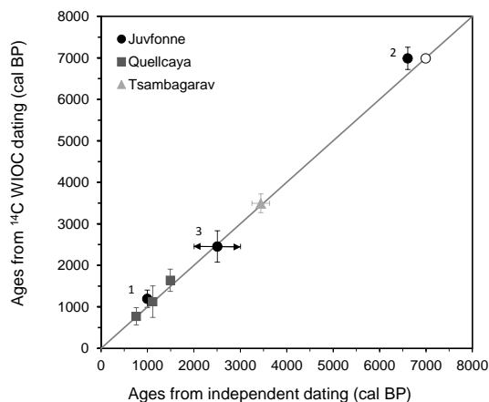
Figure 3. Scatter plot showing the ages obtained with the WIOC ^{14}\text{C} method for independently dated ice, including the conventionally ^{14}\text{C} dated Juvfonne organic-rich layers (Ødegård et al., 2016), the ^{14}\text{C} dated fly found in the Tsambagarav ice core and the Quellcaya ice dated by annual layer counting (Thompson et al., 2013). Error bars denote the 1\sigma uncertainty. Note that the Juvfonne WIOC samples and the organic-rich layers were not sampled from the exact same depth, but adjacent to each other. For the youngest (1) and oldest (2, containing the plant fragment) the ice for WIOC ^{14}\text{C} analysis was sampled below the layers whereas the third sample (3) was bracketed by two layers. For (3) the arrow thus indicates the age range between the lower and upper 2\sigma boundary of these two layers, respectively. For (2) the open circle indicates an estimated age for the according WIOC ice sampling depth based on a fit through all the conventionally dated organic-rich layers, presented in Ødegård et al. (2016).
