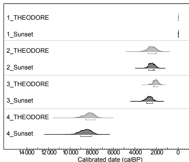
Figure 1. OxCal output for the comparability test for OC/EC separation using the THEODORE apparatus and the Sunset OC/EC analyser directly coupled to the AMS. Bars below the age distributions indicate the 1\sigma range. See Table 2 for details of the samples.
