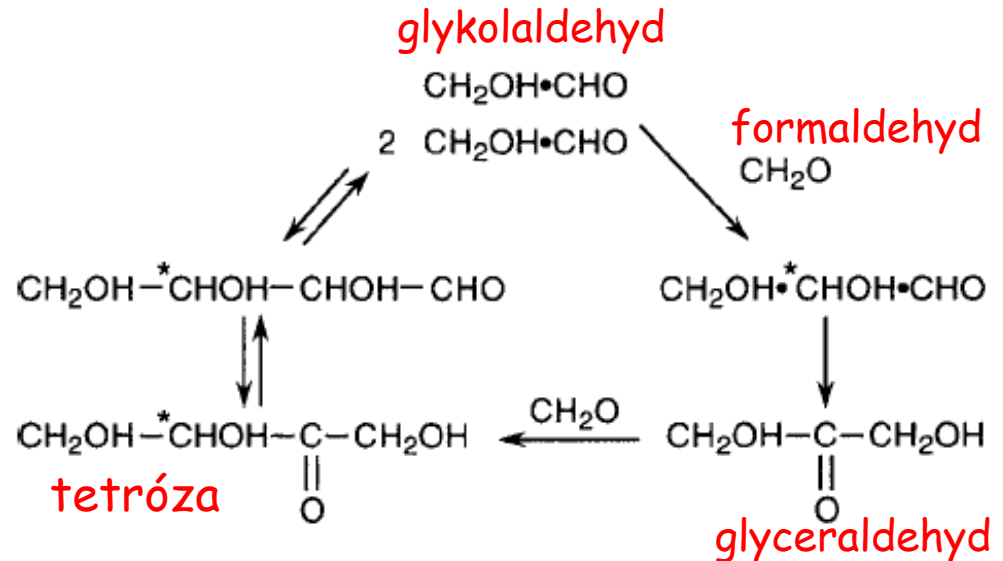
FIG. 1. The simplest hypothetical autocatalytic formose reaction cycle. In each turn of the cycle, a glycolaldehyde molecule facilitates the synthesis of a second glycolaldehyde molecule from two formaldehyde molecules. The stereochemistry at the asymmetric carbon atoms (marked with asterisks in the diagram) is not specified.
