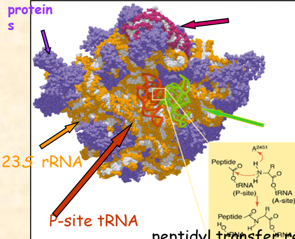
peptidyl transfer reaction:
