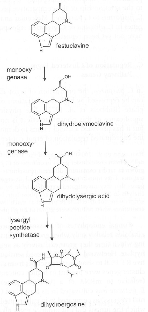
Fig. 9.6. Dihydroergot alkaloid terminal branch of the ergot alkaloid pathway. Claviceps africana follows the pathway to its completion, Claviceps gigantea does not proceed past dihydroelymoclavine
