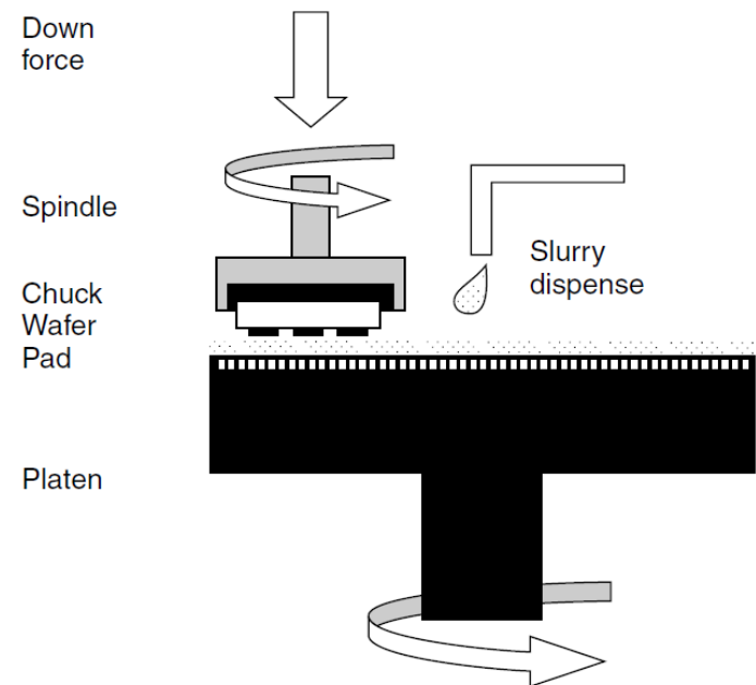
Figure 16.2 Schematic structure of a rotary CMP equipment
