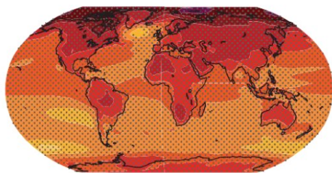
RCP 8.5
