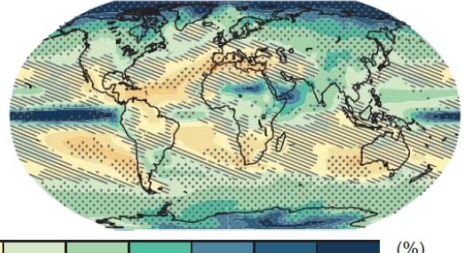
RCP 8.5
