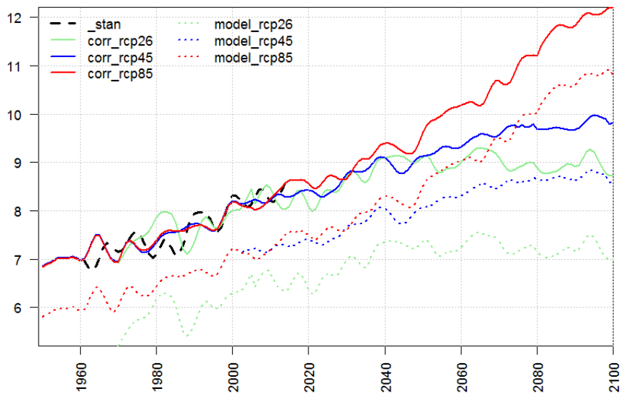
monthly-t N_YEAR
