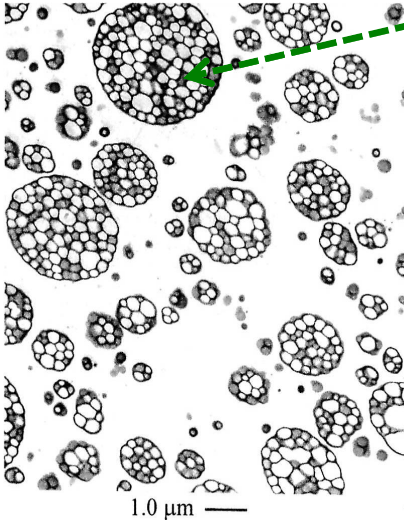
Typical HIPS particles
