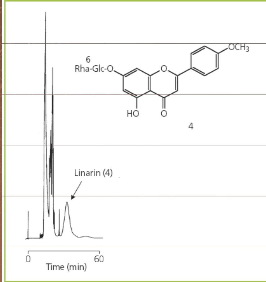
Figure 3: CCC of a methanol extract of Buddleja davidii (Buddlejaceae) leaves on a DE instrument with 17 mL coil; rotation speed: 2000 rpm; solvent system: CHCl 3 -MeOH-H 2 O 45:33:22 (mobile phase = lower phase) at a flow-rate of 1 mL/min; sample 20 mg; detection 254 nm.
