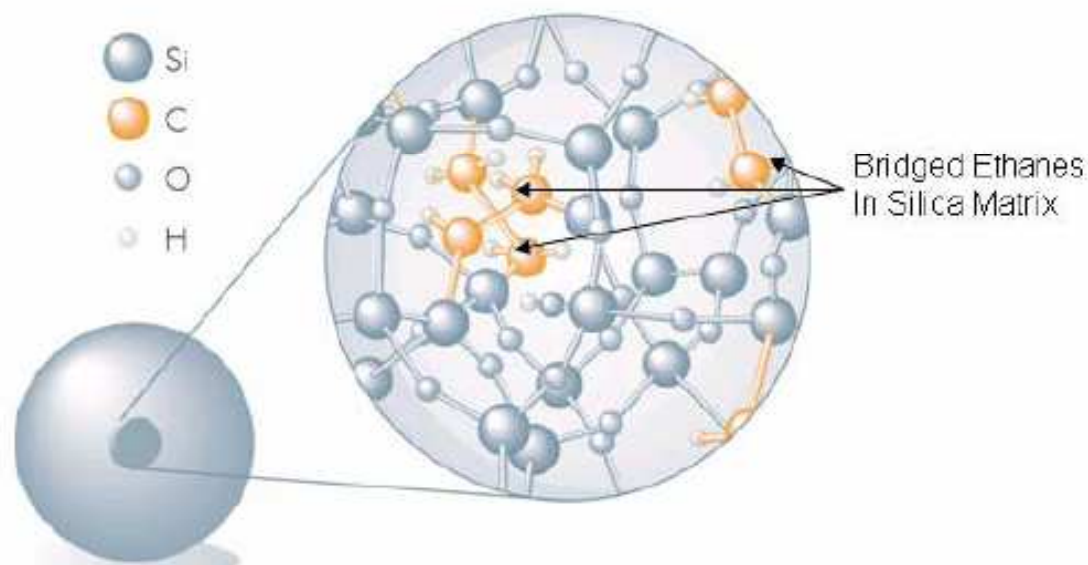
Bis(triethoxysilyl)ethane (BTEE)
