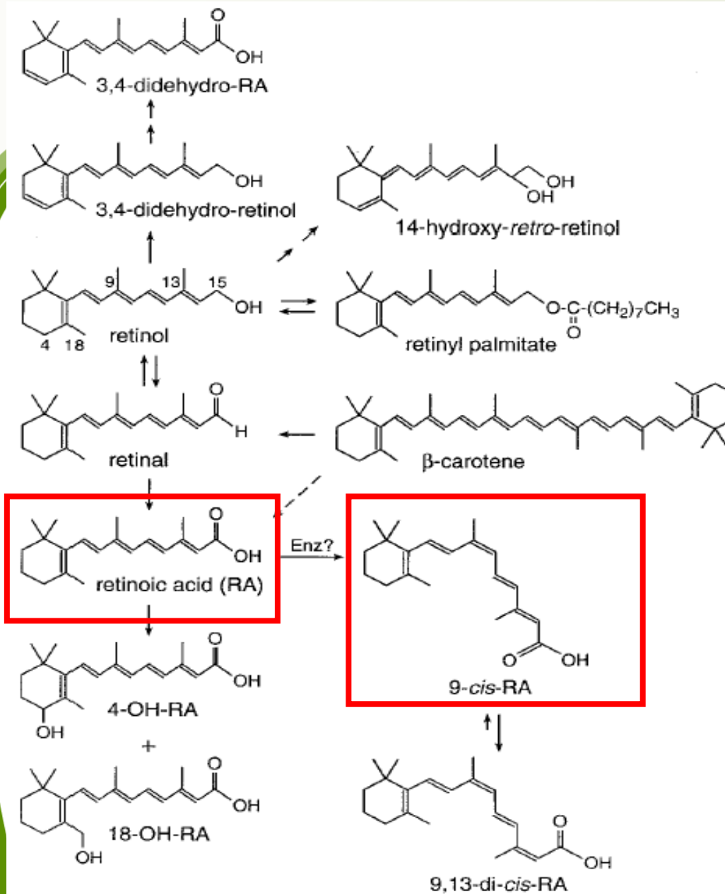
FIG. 2. Structures of naturally occurring retinoids.
