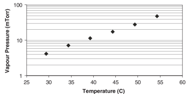
Vapour pressure data for Ta(NMe 2 ) 5
