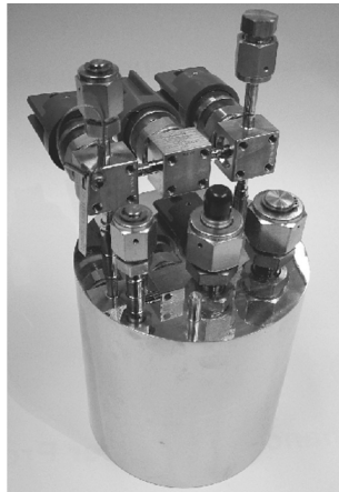
A commercial "bubbler" used to evaporate metal-organic compounds for MOCVD.
