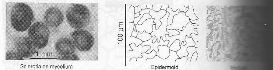
Figure 8.14: Sclerotia of Typhula ishikariensis in laboratory culture on oat meal agar. These are tracings from photographs. Cytoplasm in grey. Note the variations in wall thickness.
