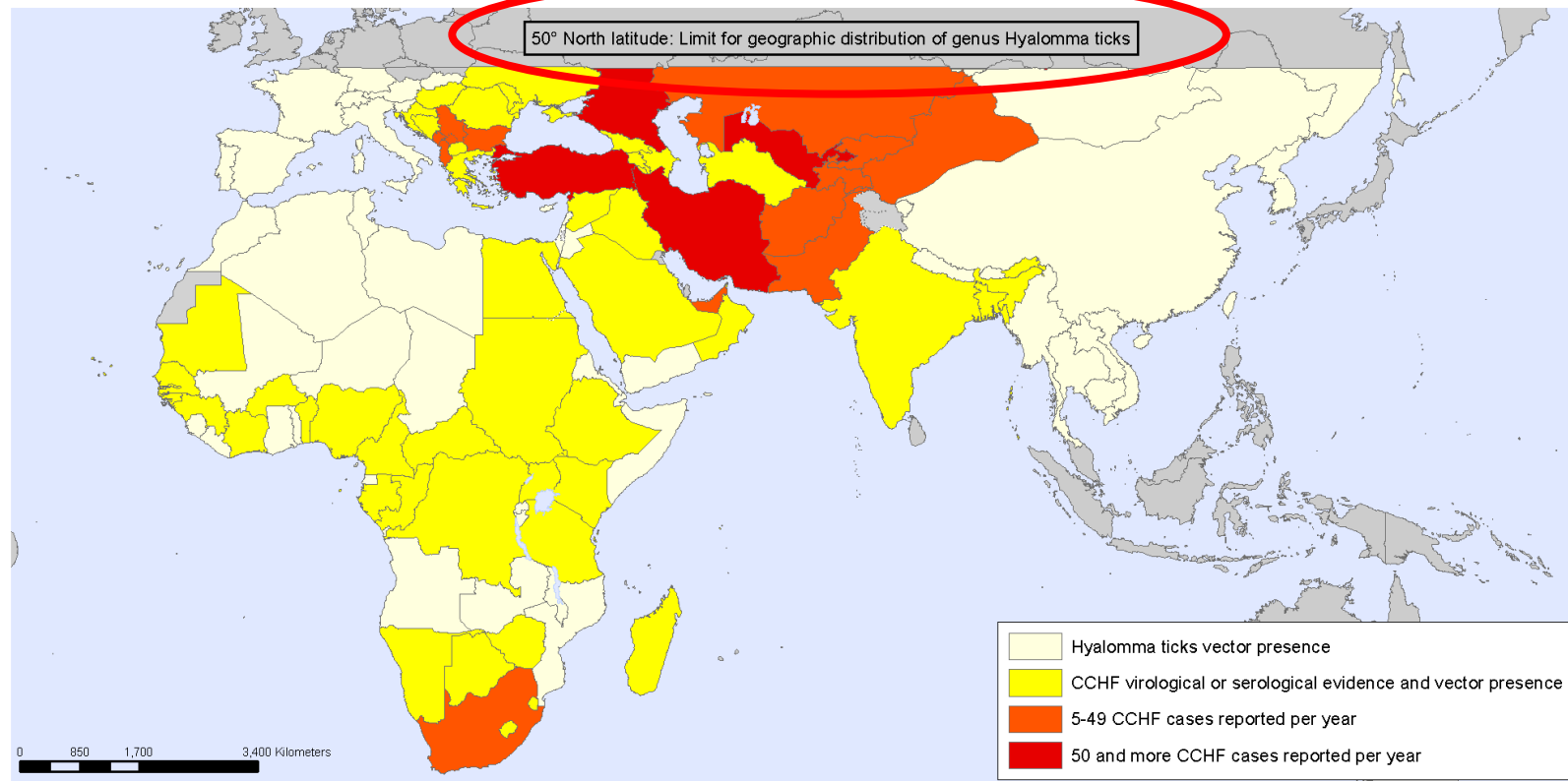
Geographic distribution of Crimean-Congo Haemorrhagic Fever
