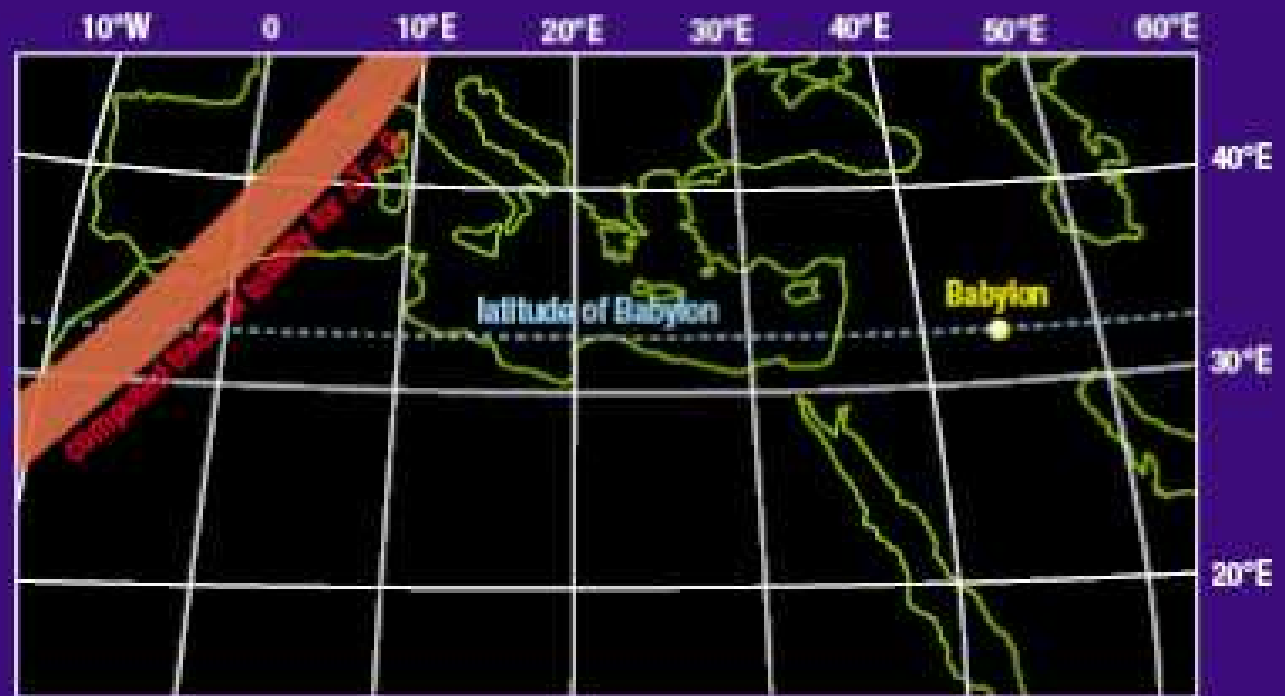
4 Computed track of totality for the eclipse of 15 April in 136 BC, assuming a fixed length of day ( \Delta T = 0 ). This track lies more than 50^{\circ} to the west of Babylon, where totality was actually observed.
