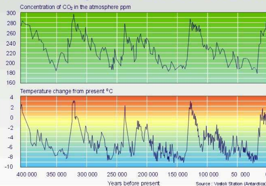
Temperature and CO 2 in the atmosphere over the past 400 000 years
