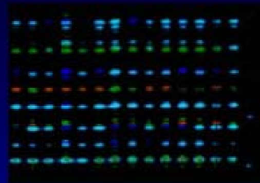
Multiplex SBE Single base extension
