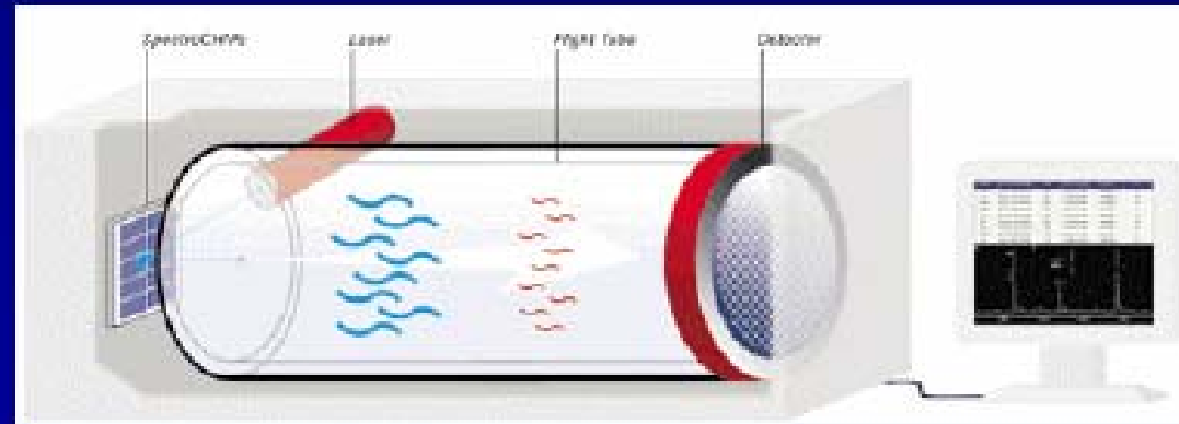
Multiplex SBE Single base extension
