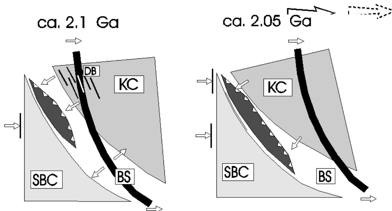
Fig. 7b-7c. Plan view of the closing stage of the Baltic sea. Intrusion of Fe-tholeiitic dykes (DB). Subduction under Svecobaltian continent. Convection cells move beneath and behind the Karelian continent.
