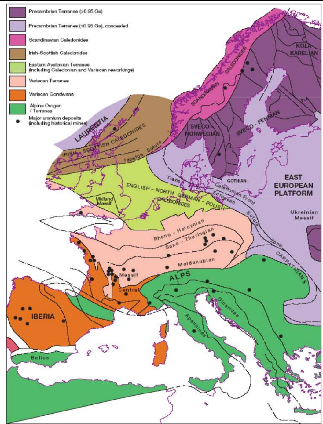
Figure 1. The 'terrane collage' of Precambrian and Phanerozoic Europe, a simplified sketch. Sutures and orogenic fronts are shown as bold lines, internal borders as thin or thin broken lines. Note that the size and shape of the terranes do not change significantly with time (approximate direction of younging is from north to south) (Reproduced with permission from Blundell et al. 1992, and Plant et al. 2003, Fig. 1, p. B229).
