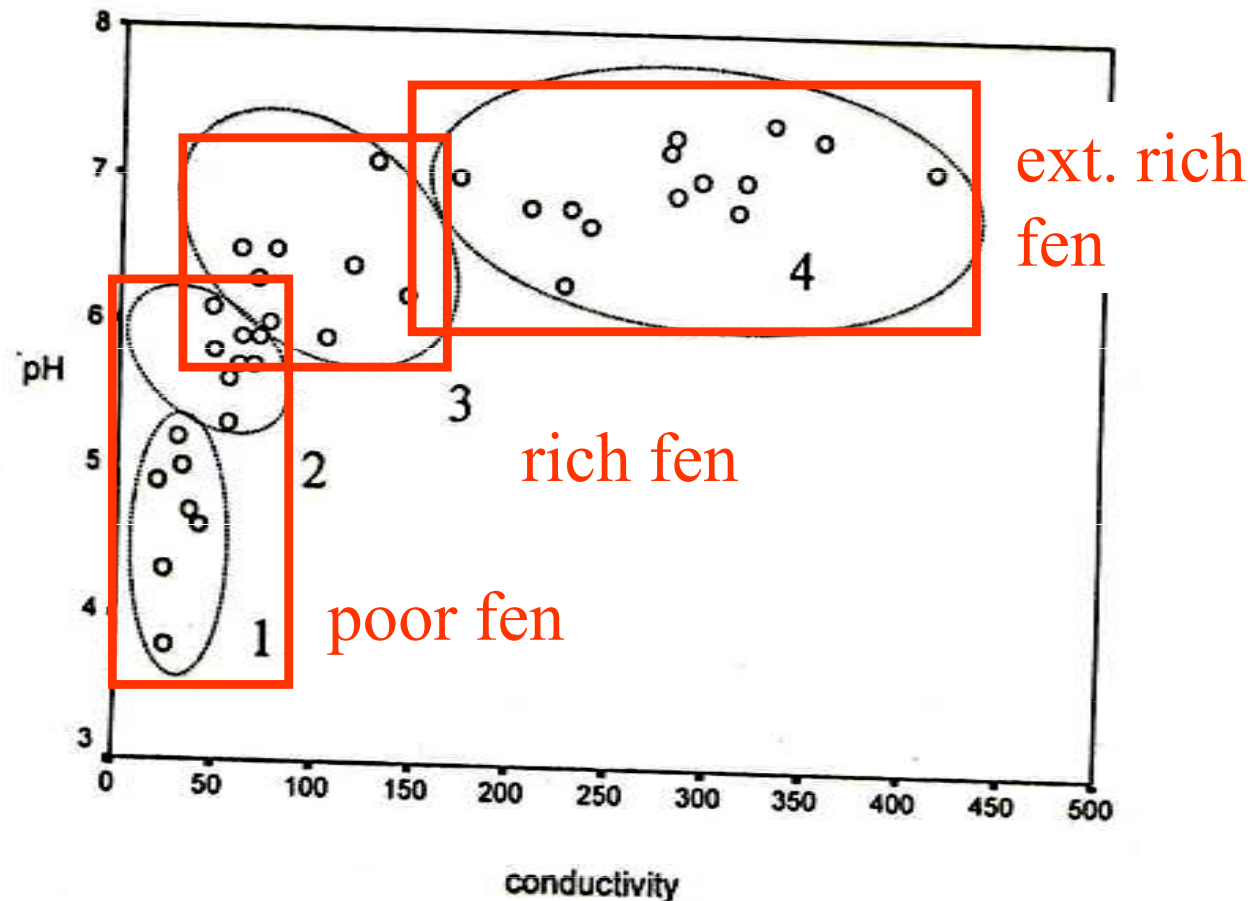
Fig. 3. Variation of pH and water conductivity ( \mu\text{S/cm/20}^\circ\text{C} ) in relation to vegetation types distinguished in the northwestern Carpathians (1 = Carici echinatae-Sphagnetum sphagnetosum fallacis ; 2 = Carici echinatae-Sphagnetum sphagnetosum flexuosi ; 3 = Sphagno warnstorffii-Eriophoretum & Caricetum goodenowii ; 4 = Valeriano-Caricetum flavae ).
