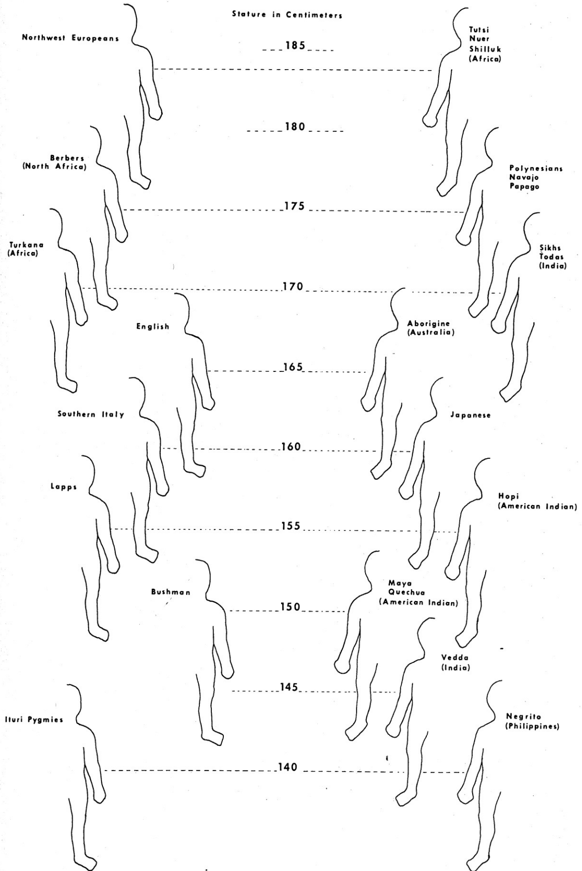
FIGURE 3-1 Diagram of stature variation between populations.
