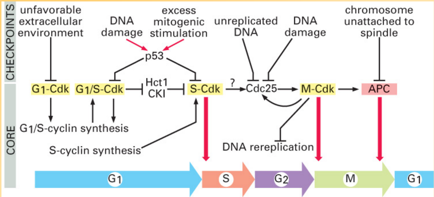
Figure 17-34. Molecular Biology of the Cell, 4th Edition.
