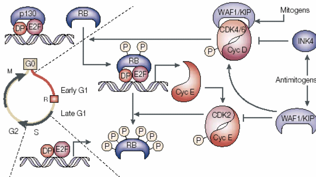
Figure 1 | Regulation of G1 and the G1/S transition. In quiescent, G0 cells, E2F–DP transcription factors are bound to p130, the principal pocket protein in these cells, which keeps them inactive. In G1, however, RB–E2F–DP complexes predominate. Mitogenic signalling results in cyclin D (Cyc) synthesis, formation of active CDK4/6–cyclin-D complexes and initial phosphorylation of RB. Partially phosphorylated RB still binds to E2F–DP, but the transcription factor is still able to transcribe some genes, such as cyclin E, presumably due to impaired repression. Cyclin E binds to and activates CDK2. It is generally accepted that CDK2-dependent phosphorylation of RB results in its complete inactivation, which allows induction of the E2F-responsive genes that are needed to drive cells through the G1/S transition and to initiate DNA replication. INK4 and WAF1/KIP proteins can inhibit CDK4/6 or CDK2 kinases, respectively, following specific antimitogenic signals. The CDK4/6 complexes can also bind WAF1/KIP inhibitors, while remaining active. This sequesters them from CDK2, which facilitates its full activation. R represents the restriction point that separates the mitogen-dependent early G1 phase from the mitogen-independent late G1 phase.
