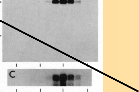
FIG. 2. Polyacrylamide gel analysis of fractions eluting from the Mono S column. A 45- \mu l aliquot of fractions 5-16 was incubated with [ \gamma - 32 P]ATP and electrophoresed through a 10% NaDodSO 4 /polyacrylamide gel. (A) Silver-stained polyacrylamide gel of purified MPF. The activity of the fractions in the cell-free assay (NEBD) and in the oocyte microinjection assay (GVBD) is shown below the gel. NEBD is expressed in units/50 \mu l. GVBD is expressed as the percentage of oocytes that underwent GVBD during a 2-hr incubation in cycloheximide (0.5 \mu g/ml). (B) Autoradiograph of the silver-stained gel shown in A. (C) H1 kinase activity of purified MPF. Mono S fractions 6-15 were assayed for H1 kinase activity. The autoradiograph of the region of the gel with histone 1 is shown. Fraction 12 had a specific activity of \approx 270 nmol \cdot min -1 \cdot mg -1 .
