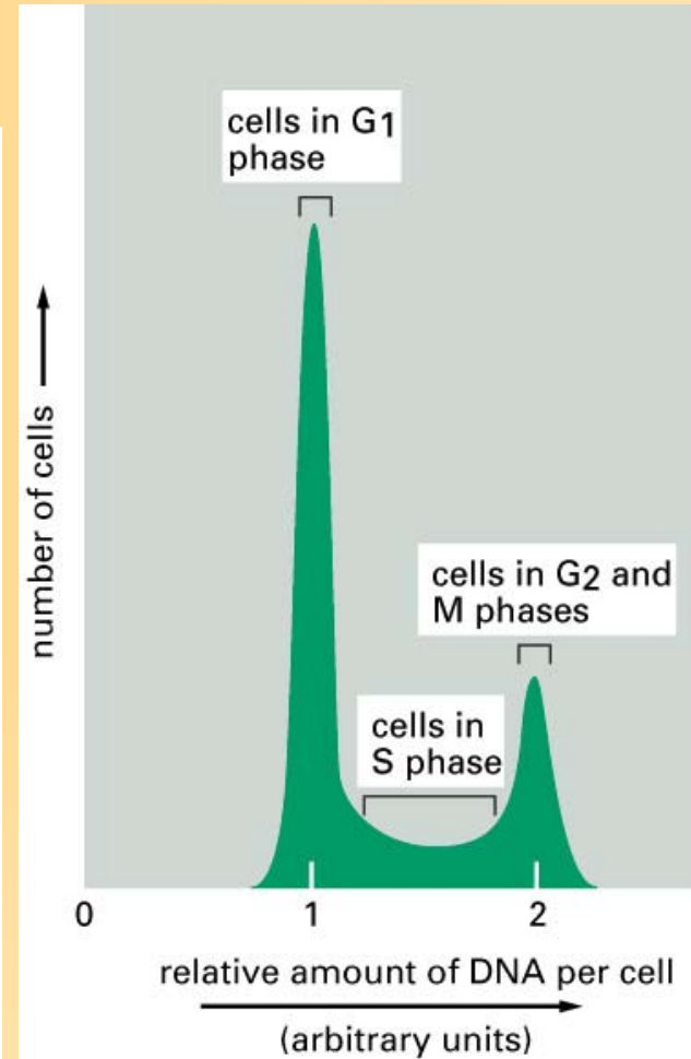
Figure 17-12. Molecular Biology of the Cell, 4th Edition.
