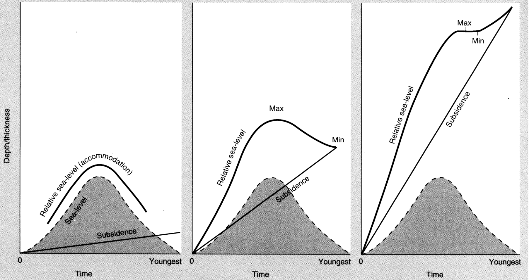
SLOW SUBSIDENCE
