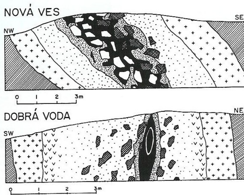
FIG. 2. Sections across the Nová Ves and Dobrá Voda pegmatites. Crosses: fine- to medium-grained granitic unit; check marks: graphic unit, open stipple: coarse-grained albite – quartz – tourmaline – mica unit, cross-hatched: blocky K-feldspar, white: blocky petalite, dense stipple pattern: albite-rich unit, black: lepidolite unit, subdivided into an outer and inner part at Dobrá Voda.
