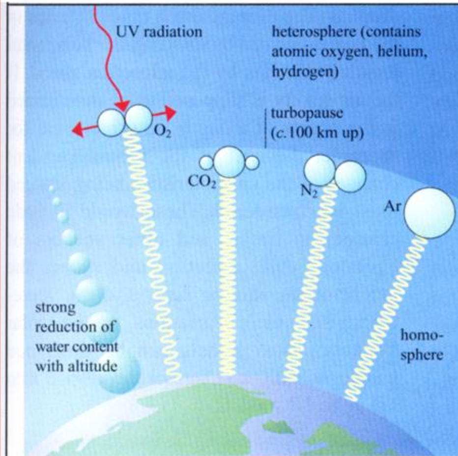
Figure 2.1.2 Composition of the atmosphere
