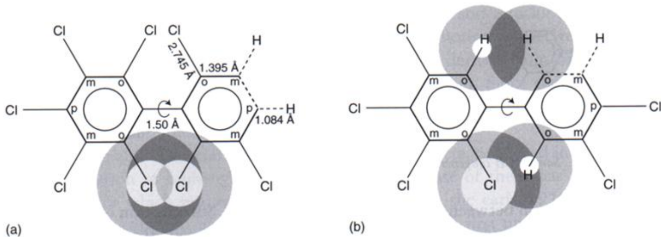
FIGURE 6.2 Planar and coplanar PCBs. Structural features of CB congeners influencing enzymatic metabolism. Areas where the principal enzymatic reaction occurs are given by broken lines. For atoms in the ortho position, the outer circle represents the area within the van der Waals radius of an atom; the dotted inner circle represents the part of this area which is also within the single bond covalent radius. The van der Waals radius indicates the maximum distance for any possible influence of an atom. The covalent radius represents the minimum distance to which atoms can approach each other. (a) Vicinal atoms in the meta and para positions. Overlapping covalent radii for two ortho Cl show that a planar configuration is highly improbable when three or four ortho Cl are present. (b) Vicinal atoms in the ortho and meta positions. Non-overlapping covalent radii for ortho Cl and ortho H show that a planar configuration causes a much lower energy barrier when chlorine atoms do not oppose each other. Reproduced from Boon et al. (1992).
