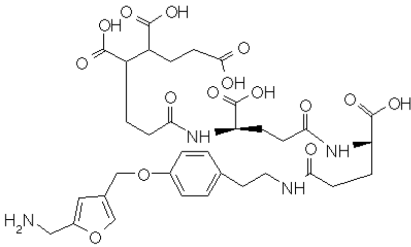
Methanofuran
