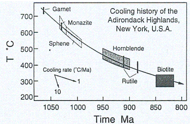
Figure 20-16. Temperature-time history for the Adirondack highlands, New York, U.S.A. Mezger et al. (1989).
