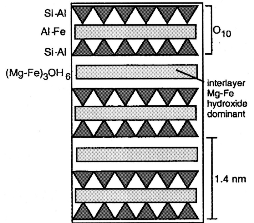
chlorite
