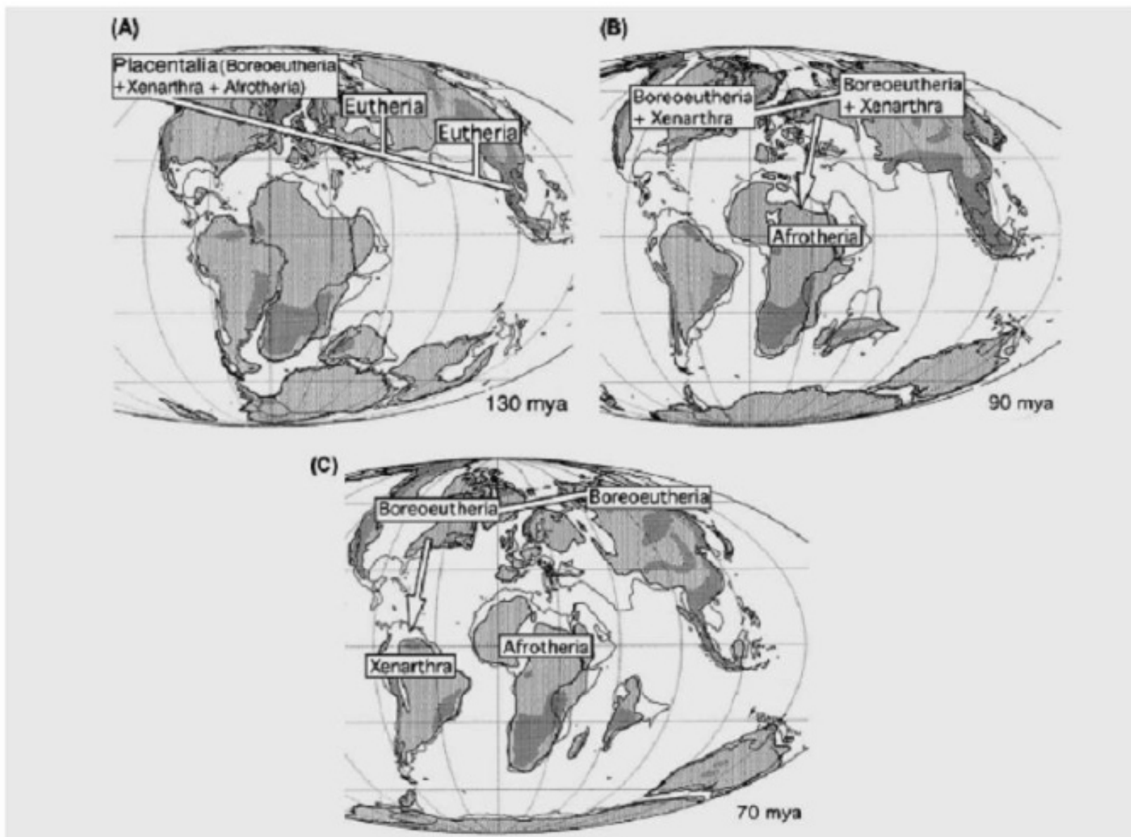
Fig. 4. Laurasian biogeographic hypothesis for the origin of Eutheria and Placentalia. See text for explanation. Base maps modified after Smith et al.
