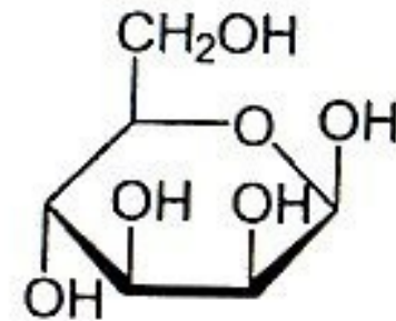
\beta -D-Mannopyranose
