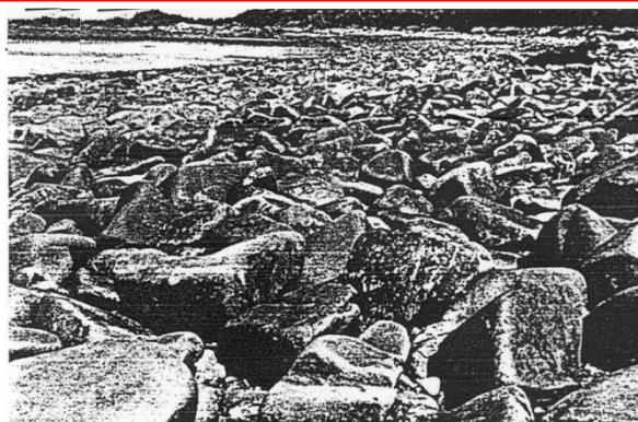
(Top) An initial, 1989 view of a heavily oiled cobble beach on Green Island, Prince William Sound, Alaska. This site was treated with a warm water wash in 1989 and by manual cleaning in 1990. The site was also fertilized in 1989 and 1990, to enhance microbial oxidation of petroleum residues. There were no treatments in 1991 or 1992. (Bottom) Condition of the same beach in 1992. Although there may be lingering hydrocarbon residues below the surface, the beach has substantially recovered through the combined actions of cleanup and natural processes (photos courtesy of Exxon Co., Houston, TX).
