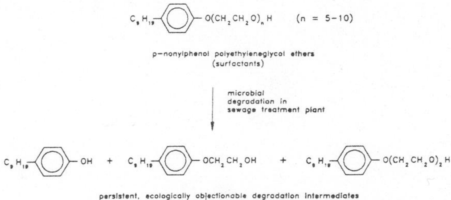
Figure 2.9 Example of a group of widely used chemicals which, as a consequence of biological waste water treatment, are converted into persistent objectionable degradation intermediates (from Giger et al., 1984).
