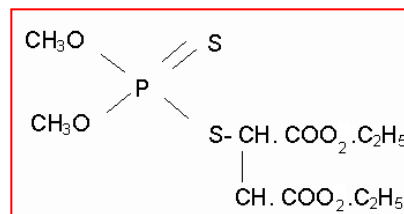
Malathion
