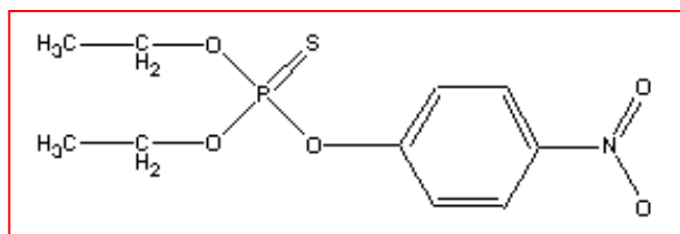
Parathion
