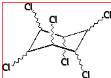
Lindan
