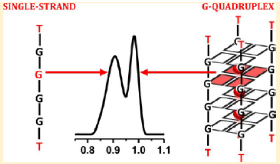
parallel tetramolecular
