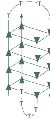
antiparallel bimolecular
