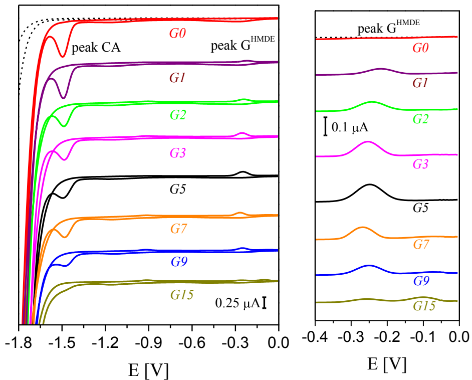
Cyclic voltammetry on HMDE
