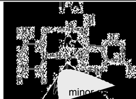
adenine (A)
