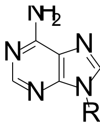
adenine (A)
