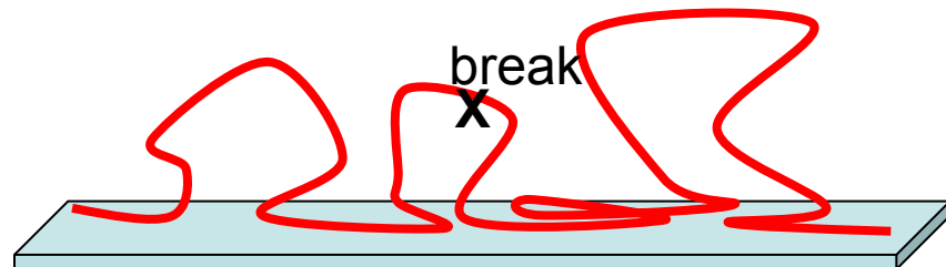
intDNA with intercalator
