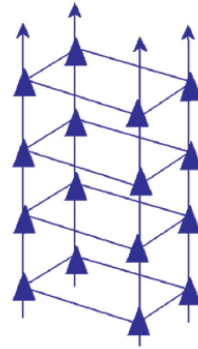
parallel tetramolecular
