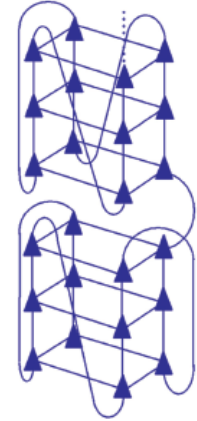
parallel monomolecular (telomeric DNA)
