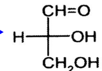
D-glyceraldehyd D-glycero
