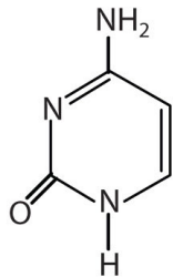
Cytosine (C) both DNA and RNA
