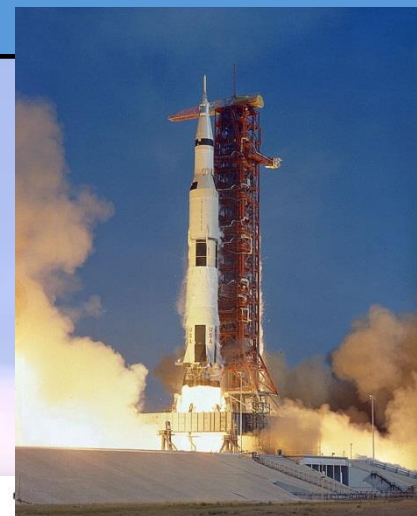
Average Radiation Doses of the Flight Crews for the Apollo Missions
