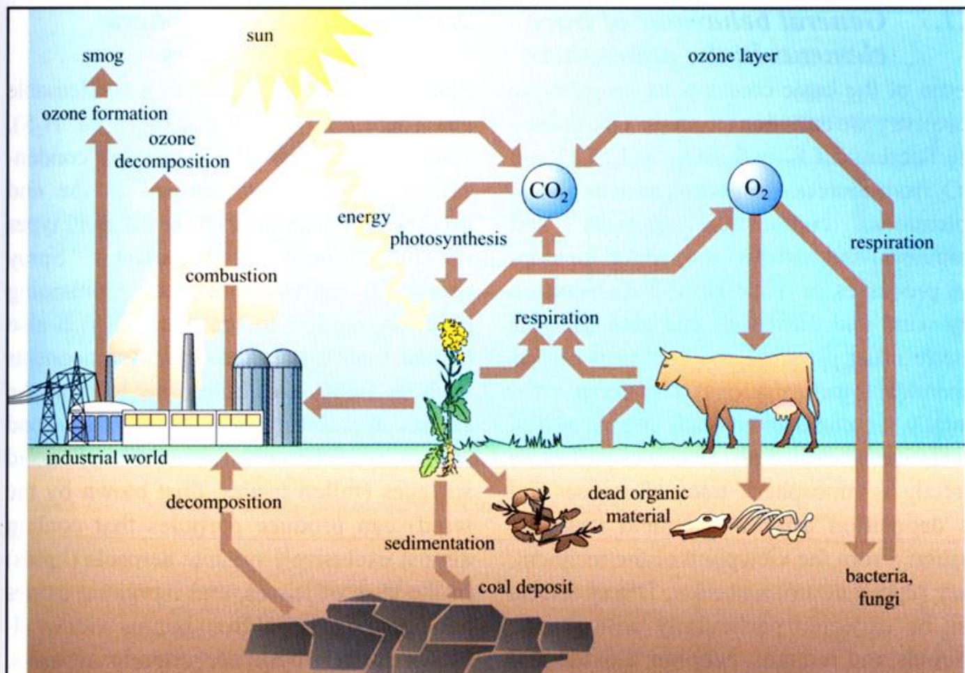
Figure 2.1.5 Linking the carbon and oxygen cycles
