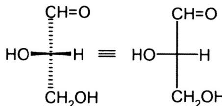
L-glyceraldehyd
