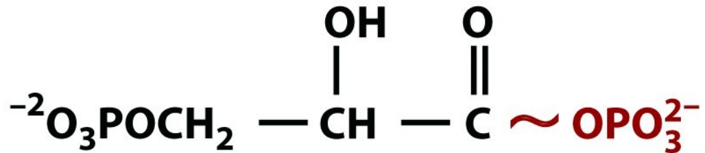
1,3-Bisphosphoglycerate
