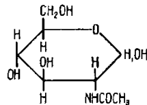
N-Acetyl-D-Glukosamin
