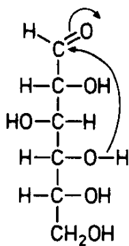
D-Glucose
