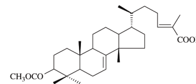
3-O-acetyl-3-epi-(iso)masticadienonic acid
