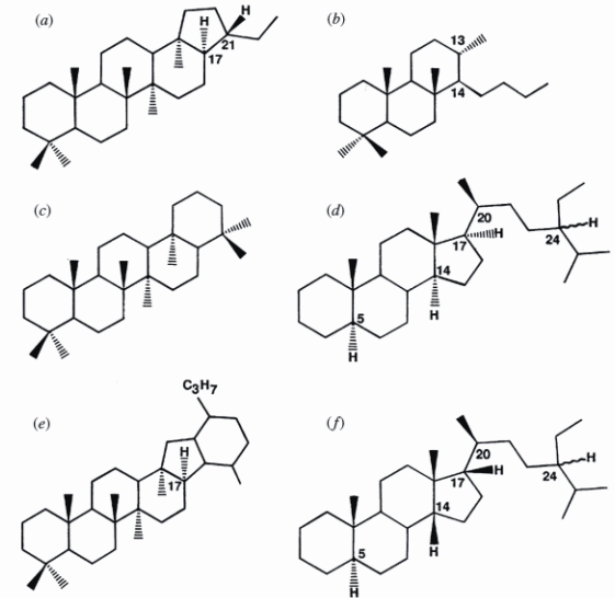
Figure 2. Molecular structures of some typical biomarkers found in the C_{15s} alkane fraction. Steranes are represented by (d) 5\alpha(H) , 14\alpha(H) , 17\alpha(H) -20S-24-ethylcholestane (abbreviated to 29 \alpha\alpha\alpha S) and (f) 5\alpha(H) , 14\beta(H) , 17\beta(H) -20S-24-ethylcholestane (abbreviated to 29 \alpha\beta\beta S). (b) C_{27} -13 \beta(H) , 14\alpha(H) -tricyclopolyprylene (abbreviated to 23/3) is generally the
