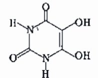
5,6-Dihydroxyuracil (5,6-diOH-Ura)
