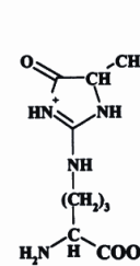
Methylglyoxal-arginine
