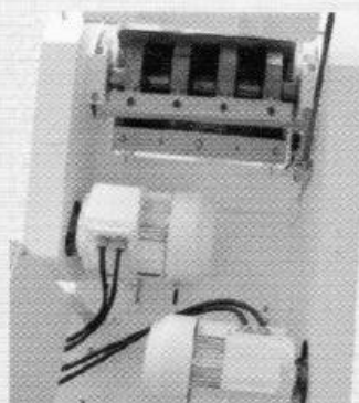
4.10 Pohon a rotor driiča DP 30 – 350/630
