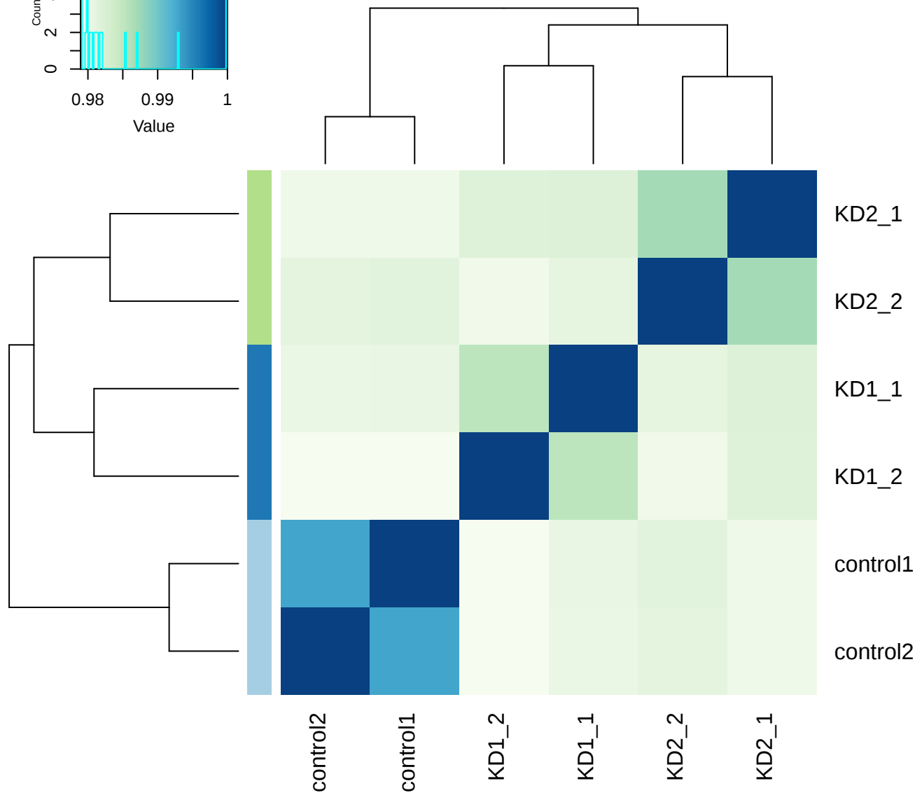
Sample to Sample Correlation (Log2)
