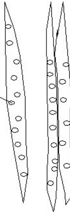
TRACHEIDS
