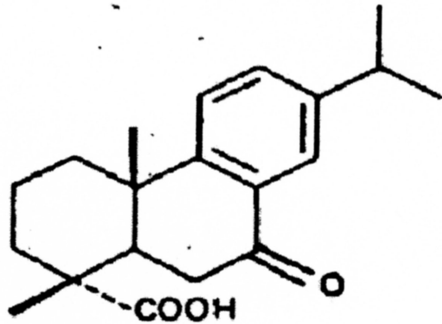
7-oxodehydroabietic acid
