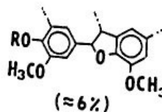
α-arylether
