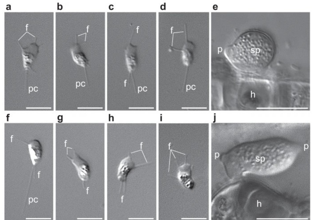
a–e Life cycle stages of Sanchytrium tribonematis . f–j Life cycle stages of Amoeboradix gromovi . a–d, f–i Amoeboid crawling zoospores with filopodia (f) and posterior pseudocilium (pc). g–i Zoospores with retracted pseudocilium. e, j Sporangium (sp) with one (e) or two (j) papillae (p) on the host (h) surface. Scale bars: a–d, f–i , 5 \mu\text{m} ; e, j , 10 \mu\text{m} .
