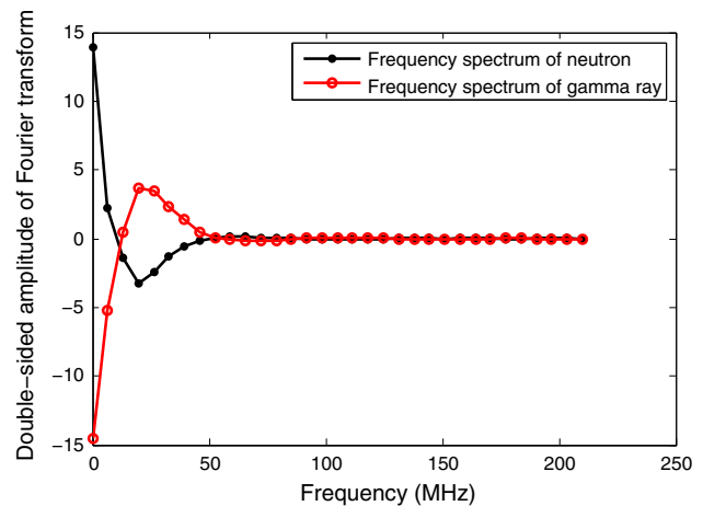
Fig. 23 The double-sided amplitude spectra of the \gamma -ray and neutron events shown in Fig. 22, applying a 64-point FFT. The pulses are obtained using DC440 digitizer (12-bit resolution, 420 MS/s)
