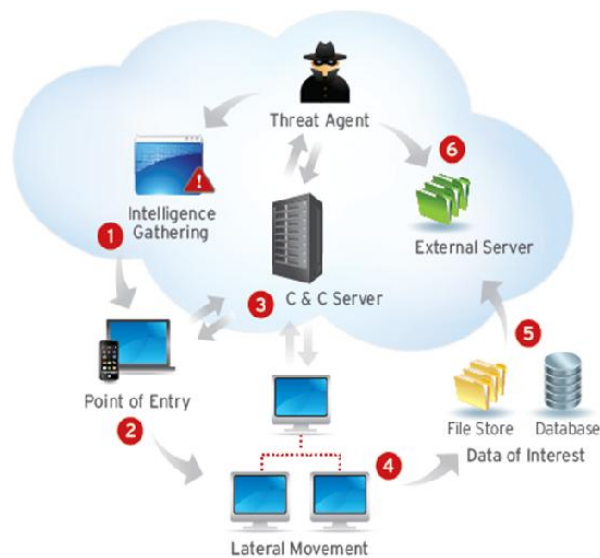
Fig. 2. Typical steps of APT attack.
