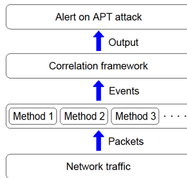
Fig. 1. Architecture of our proposed approach.
