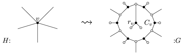
Fig. 7. The vertex-gadget of Lemma 5.3, replacing vertices of H with \{1, 3\} -regular parts in G .
