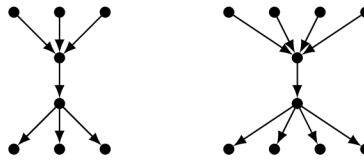
Fig. 5. Digraph H from the proof of Theorem 4.12 .
