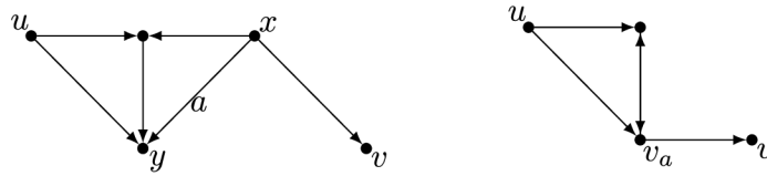
Fig. 2. Arc contraction: digraphs D (left) and D/a .
