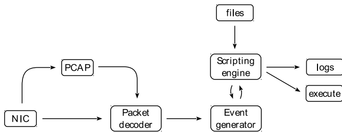
Figure. 7. Bro architecture.
