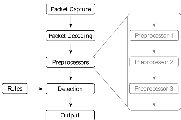
Figure 4. Snort architecture.
