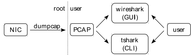
Figure. 2. Wireshark architecture showing privilege separation.
