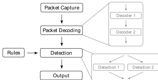
Figure 6. Suricata's architecture.
