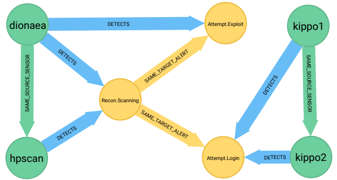
Fig. 2. Graph sample depicting 4 sensors, 3 alert types, and 3 relation types.
