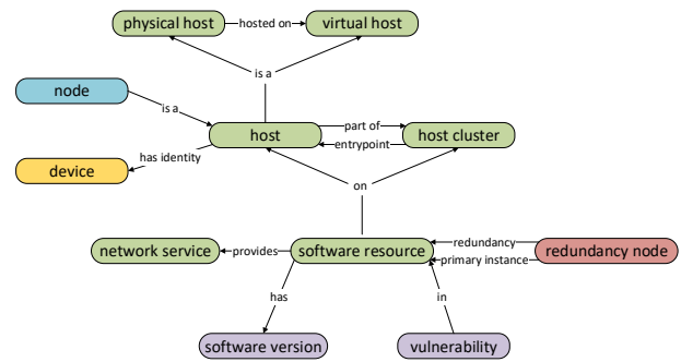
Figure 2: Host Layer
