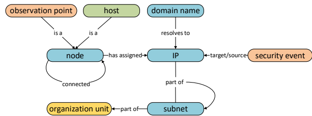
Figure 4: Network Layer
