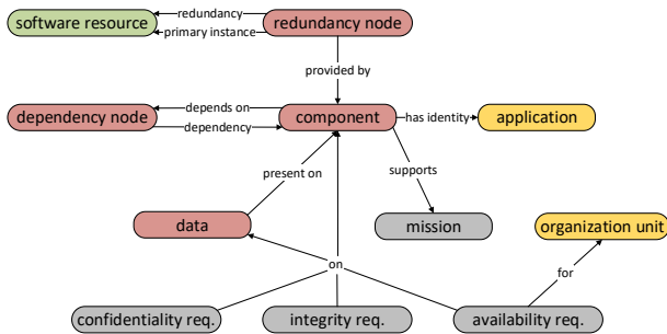
Figure 3: System Layer
