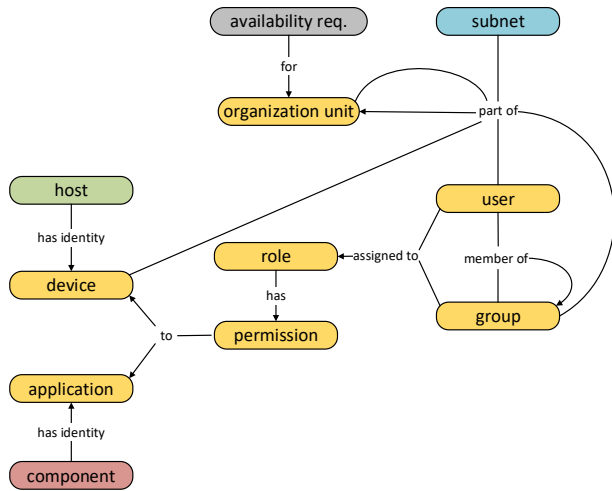
Figure 6: Access Control Layer
