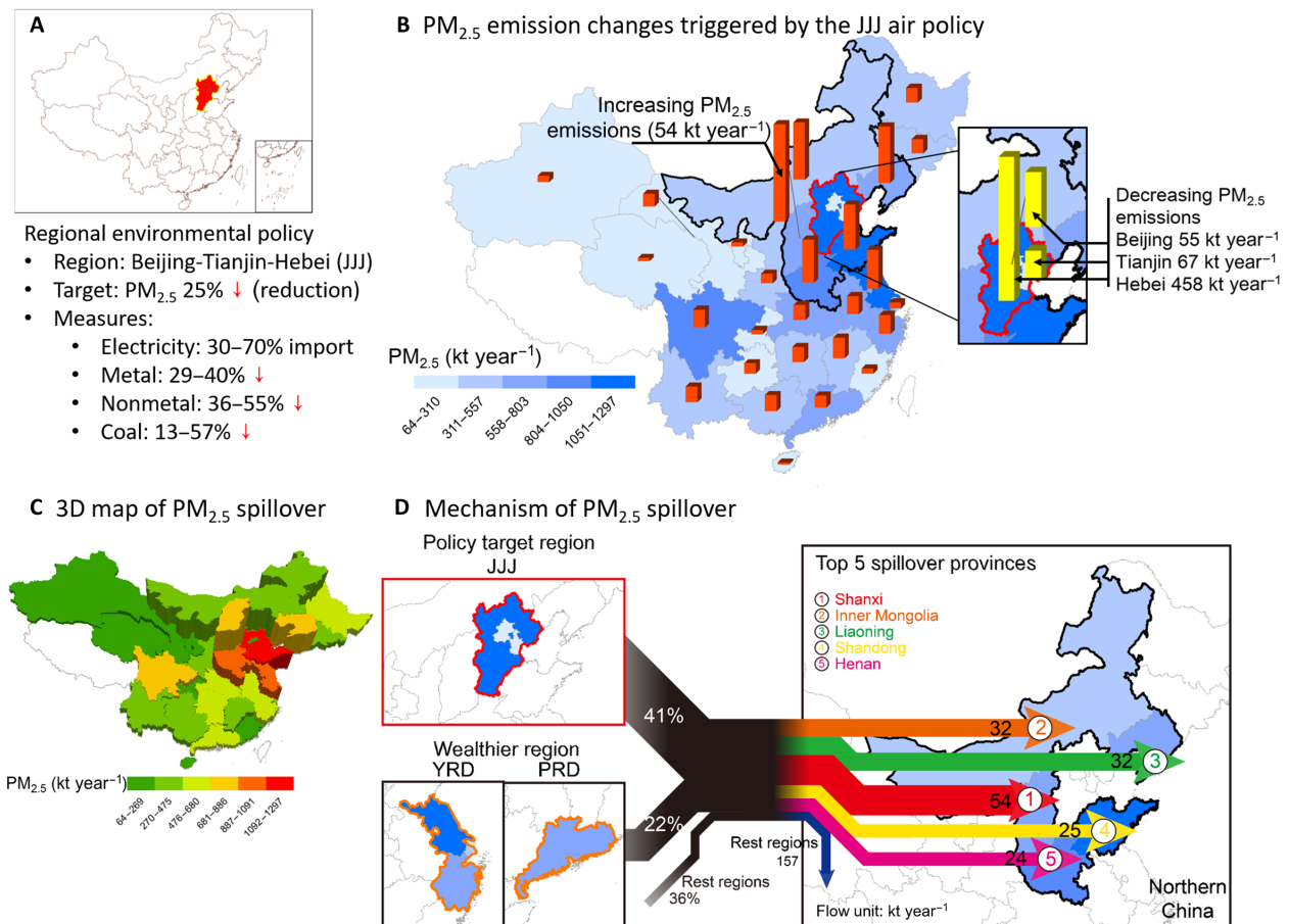
Fig. 1. Primary PM 2.5 emission changes triggered by the JJJ clean air policy. (A) JJJ clean air policy. Red part shows the JJJ region. (B) Primary PM 2.5 emission changes triggered by the JJJ clean air policy, with regions shaded according to primary PM 2.5 total emissions. Yellow bars show the reduction in primary PM 2.5 emissions in JJJ, and red bars show the increase in primary PM 2.5 emissions in the rest of China. (C) Three-dimensional map of primary PM 2.5 spillover from JJJ to other regions. (D) Mechanism of primary PM 2.5 spillover from the policy target region (JJJ) and wealthier regions (YRD and PRD) to northern China. The colored arrows show the direction and amount of primary PM 2.5 spillover to the provinces of Shanxi, Inner Mongolia, Liaoning, Shandong, and Henan.
