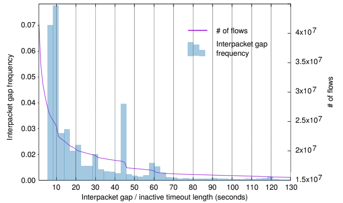
Fig. 1. Impact of interpacket gaps and inactive timeouts on number of flows. (Dataset1, TCP)
